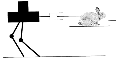
Figure 6: Spring Turkey with virtual dog track bunny mechanism.
